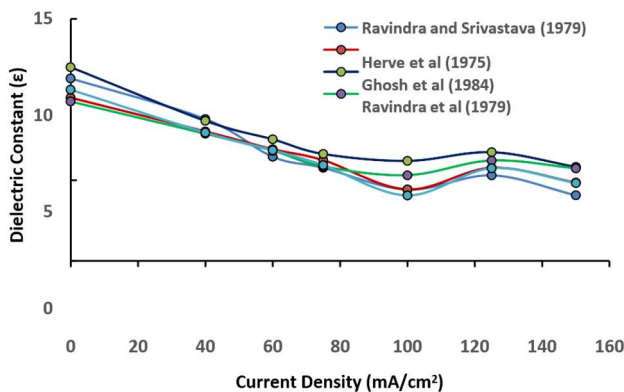
Fig. 3. Variation of dielectric constant ( \epsilon ) with current density for five models.
